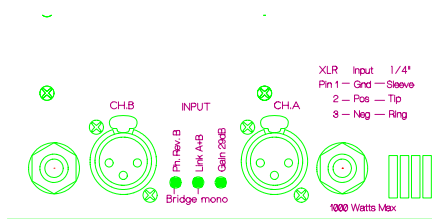
Figure 5. Rear panel connectors
