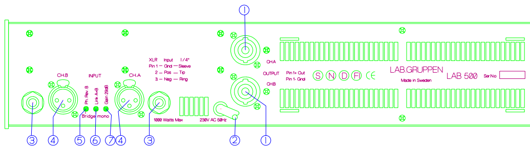
Figure 2. Rear panel
