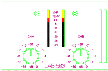
Figure 12. Front indicators
