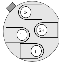
Figure 9. Speakon connector
