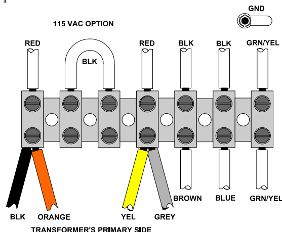
Figure 14. 115 VAC wiring
