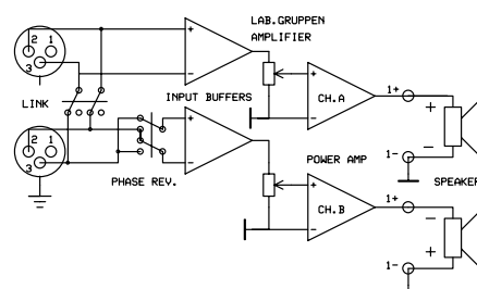
Figure 11. Stereo reverse mode
