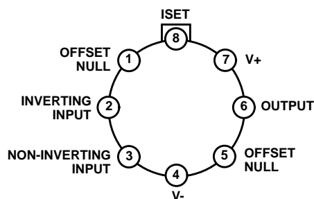
8 LEAD METAL CAN PACKAGE (CAN) MIL-STD-1835 MACY1-X8 TOP VIEW
