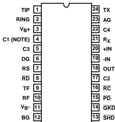
HC-5502B1 (PDIP, SOIC) TOP VIEW
