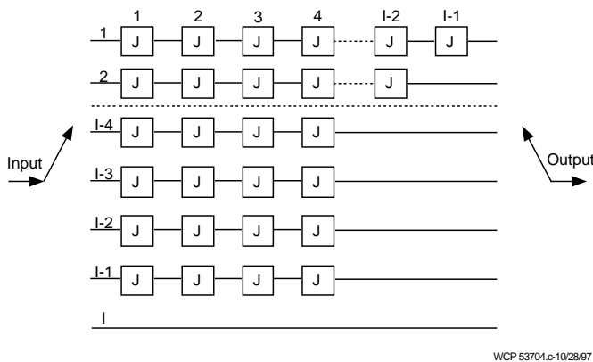
Figure 12. De-Interleaver
