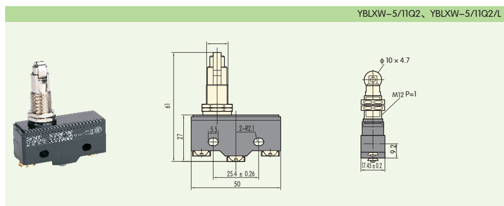
YBLXW-5/11N1、YBLXW-5/11N1/L
