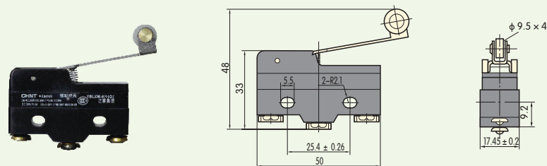
YBLXW-5/11G1、YBLXW-5/11G1/L
