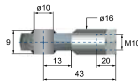
4-M10 Gelenkkopf Spherical end bearing Joint articulé • Forcella snodata Charnela macho articulada
