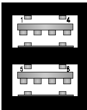
USB 2.0 Connector
