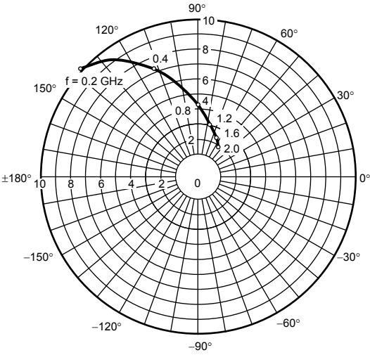
S 21e V CE = 8 V I C = 5 mA T a = 25°C
