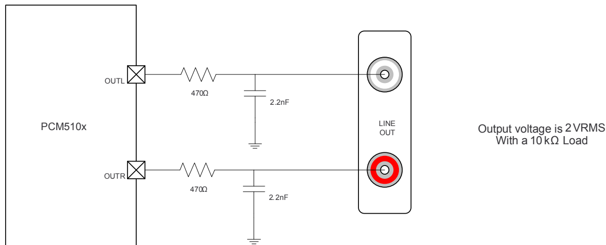
Figure 39. Recommended Output Lowpass Filter for 10kΩ Operation
