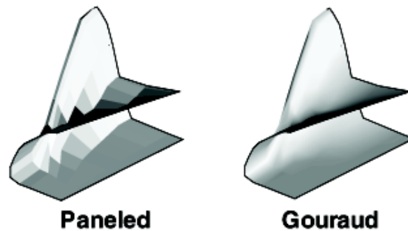
Figure 13-2. A comparison of the paneled (left) and Gouraud (right) lighting effects.
