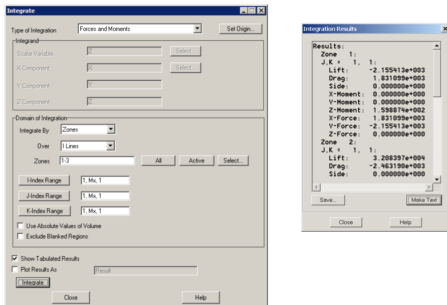
Figure 22-13. The Integration dialog and the integration results for calculating the lift and drag for the data shown in Figure 22-12 .
