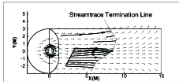
Figure 15-2. A streamtrace termination line drawn through surface streamlines. This figure was created with demo file cylinder.plt . This file is located in your Tecplot 360 distribution under the examples/2D subdirectory.
