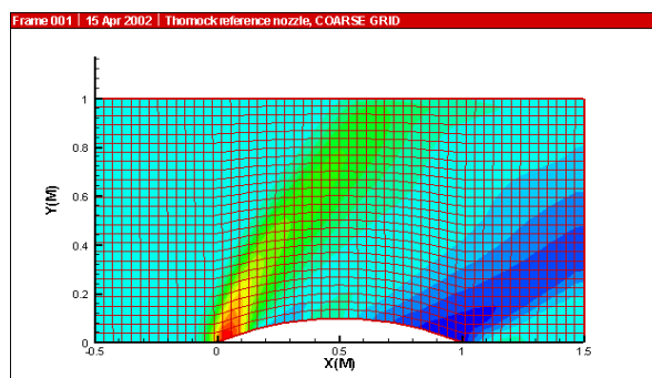
Figure 22-8. An internal flow solution. This file, intflow.lpk , is located in your Tecplot 360 distribution under the examples/2D subdirectory.
