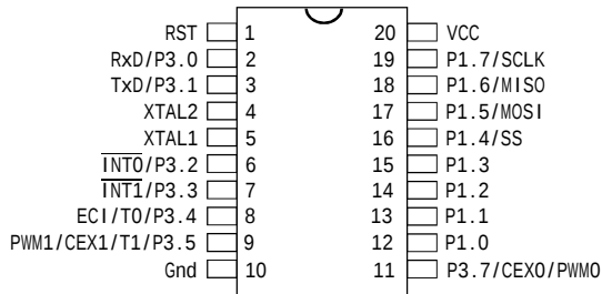
STC12C2052
