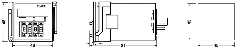
H5CN-B + Y-48 Adapter
