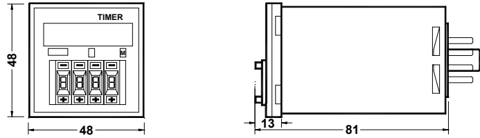
H5CN-B + Y-48 Adapter
