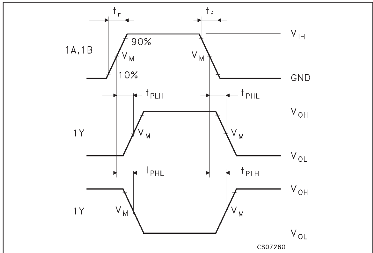
WAVEFORM: PROPAGATION DELAY ( f=1\text{MHz} ; 50% duty cycle)
