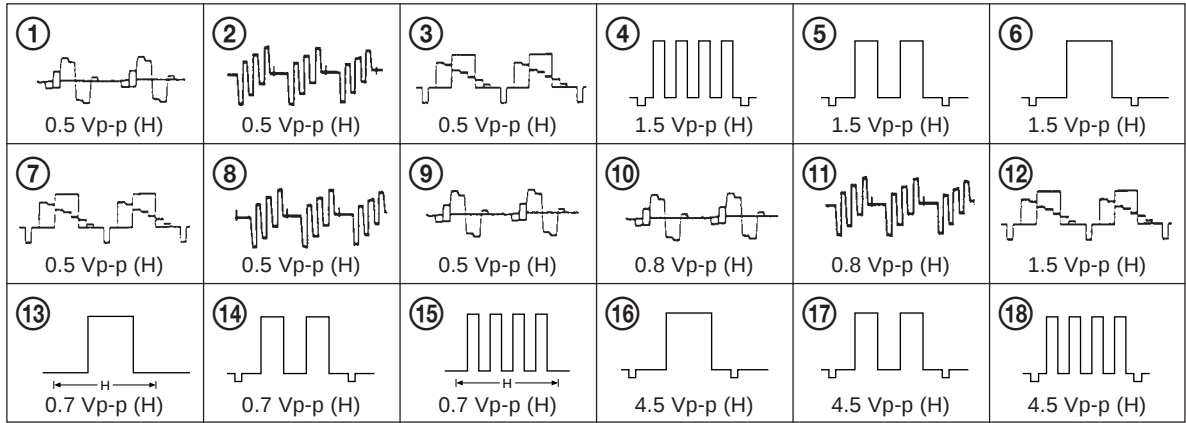
• A (3/3) BOARD WAVEFORMS
