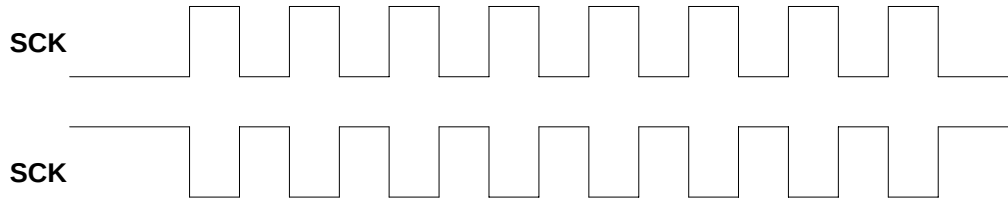
Figure 10-3. The Two SCK Directions of SIO Master Operation
