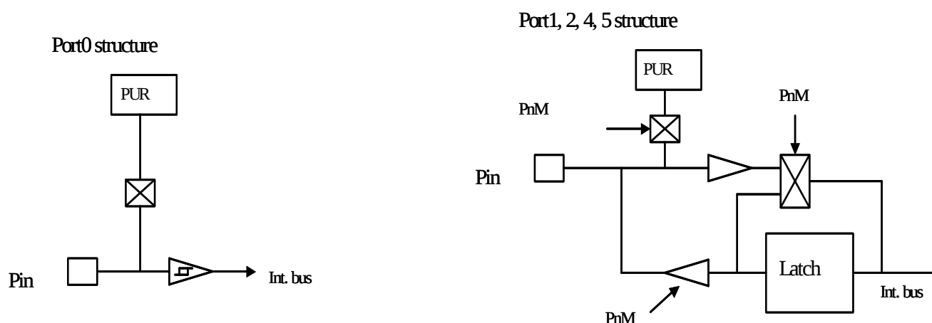
Figure 11-1. The I/O Port Block Diagram
