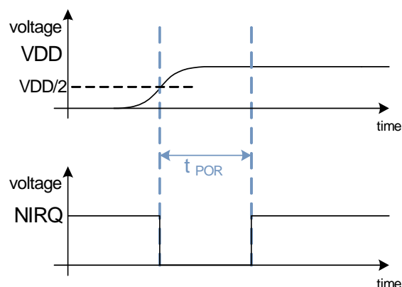
Figure 13. Power-up, NIRQ
