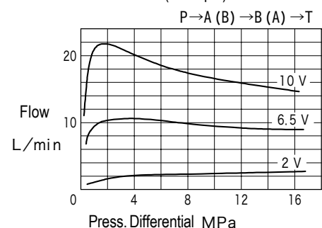
Pressure Differential-Flow Characteristics (Example)
