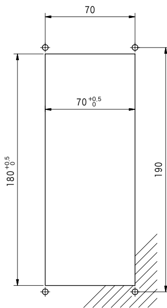
Panel Cut Dimensions
