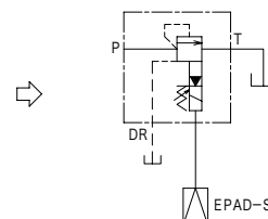
EPAD with Proportional Relief Valve
