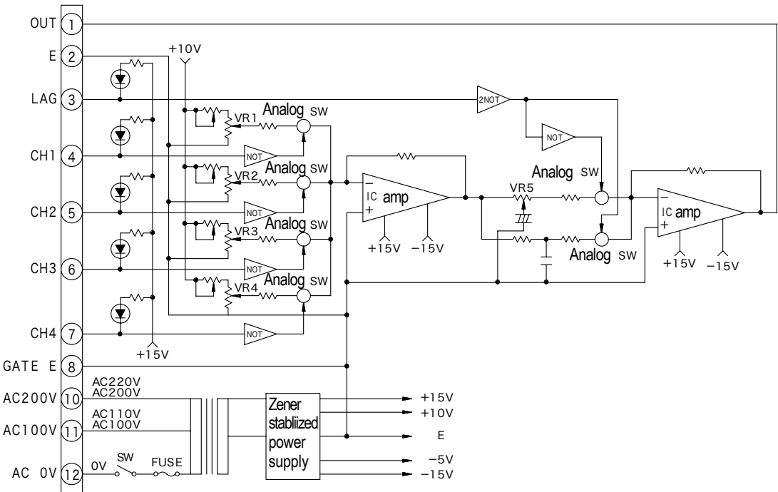
Block Diagram
