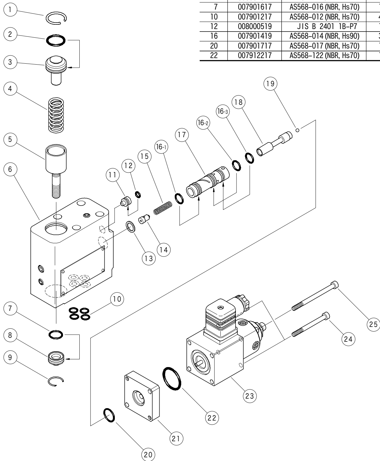
O-Rings
