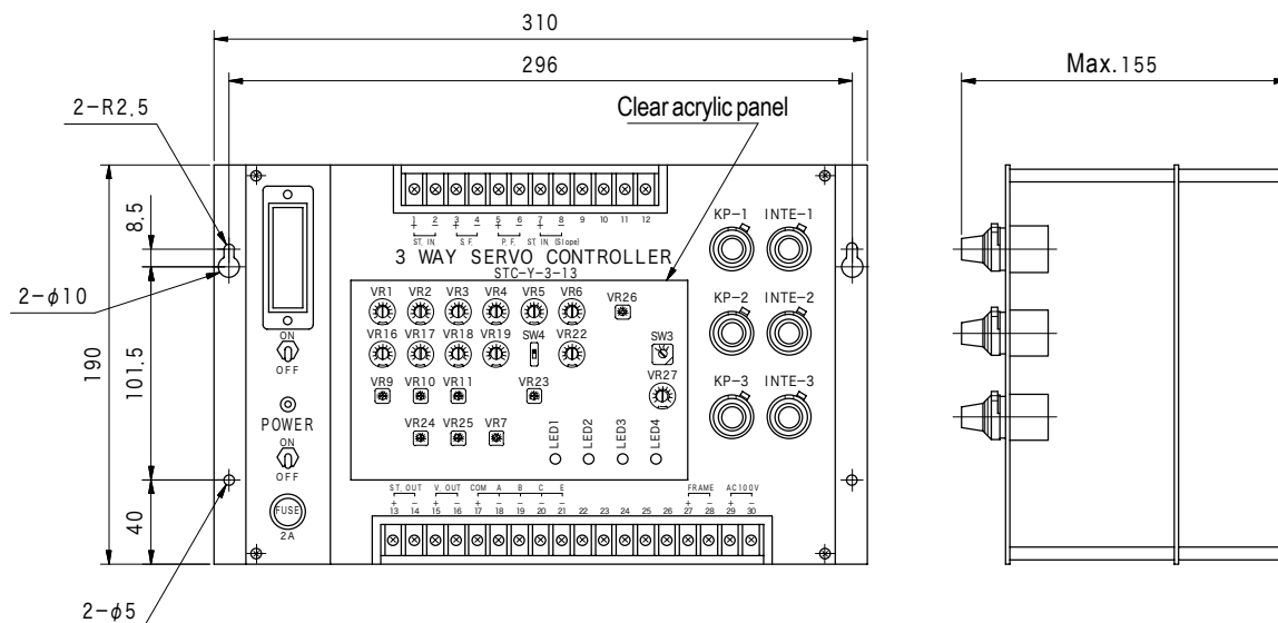
Mounting Dimensions
