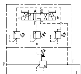
Conventional Circuit
