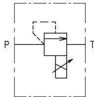
Functional Symbol
