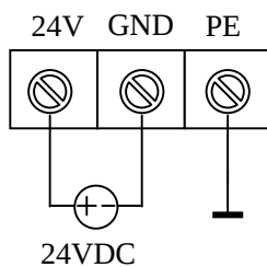
图2 PIO-DI20DO12R2 一体机电源端子图
