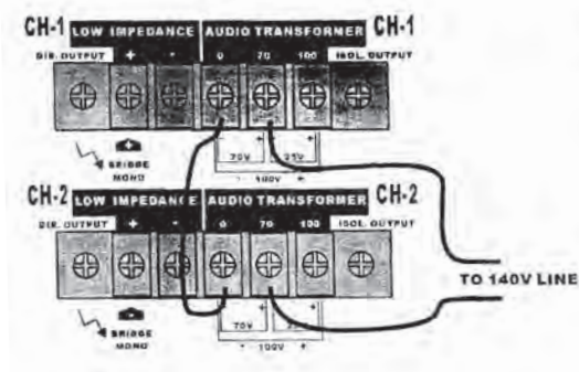
140 volt line output connection, bridge mono mode
