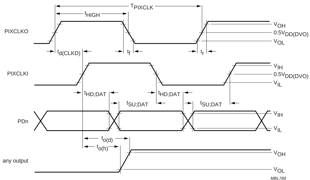
Fig.48 Input/output timing specification.
