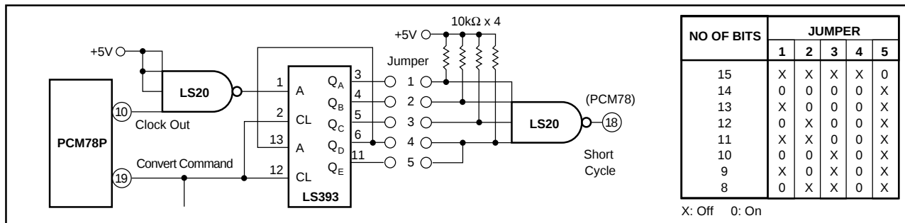
FIGURE 11 . Short Cycle Circuit.
