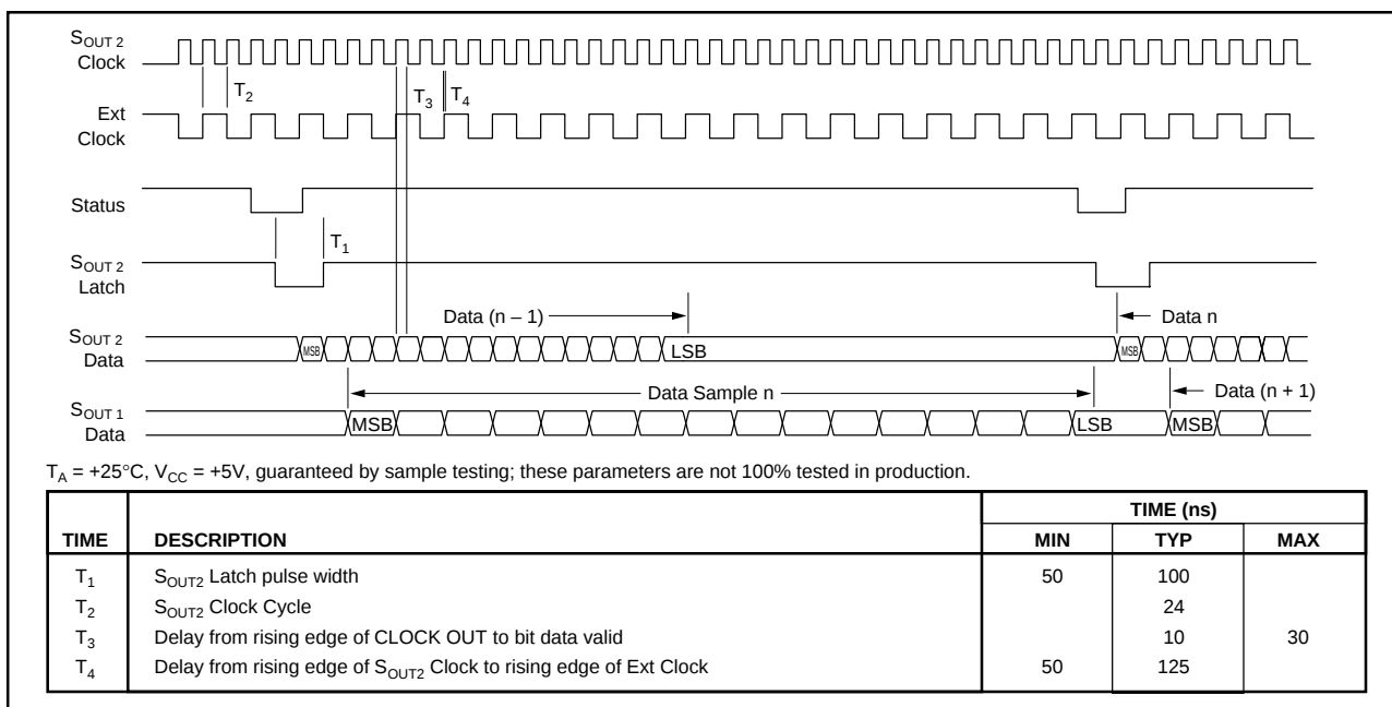
FIGURE 9. Timing when using S_{OUT2} Latch.
