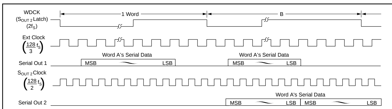
FIGURE 10. Application Example of S_{OUT2} Operation.
