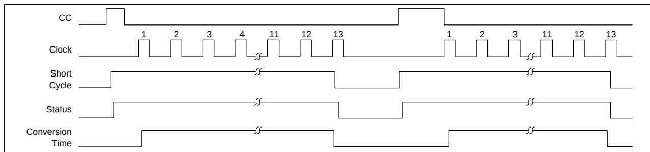
FIGURE 12. Short Cycle Operation Timing.
