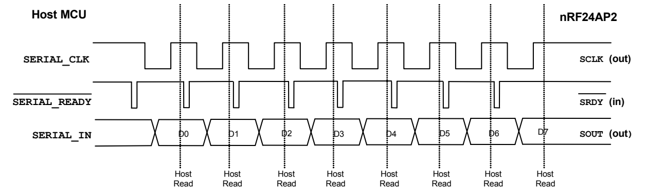
Figure 21. nRF24AP2 → host transaction
