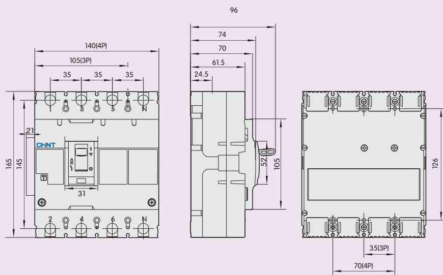
NM7-250
