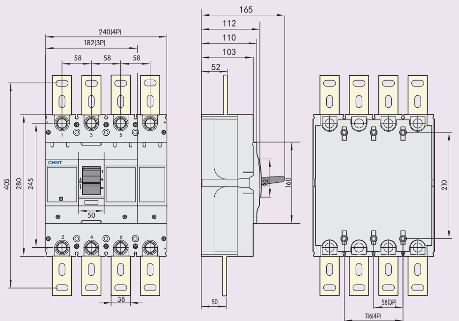
NM7-630
