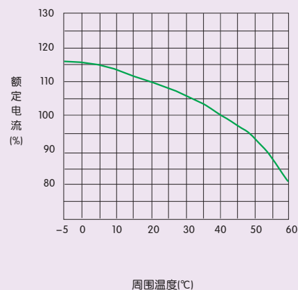
图4 NM7-63(40A~63A)/NM7-125(40A~125A)温度补偿曲线
