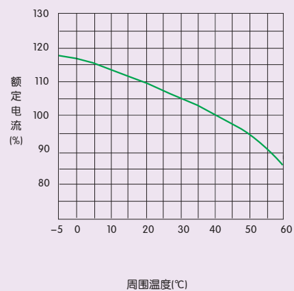
图2 NM7-63(10A~32A)/NM7-125(16A~32A)温度补偿曲线
