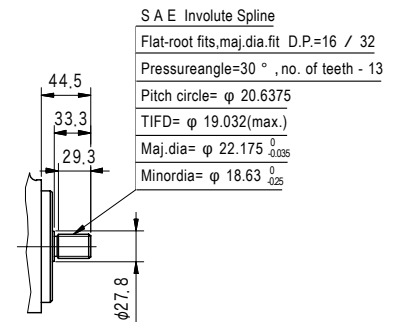
No.11 Spline Shaft End
