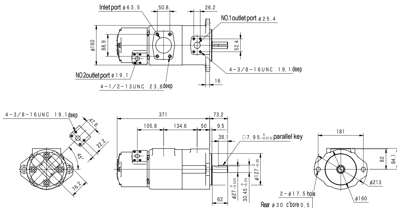
Foot Mount
