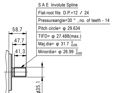
No.11 Spline Shaft End
