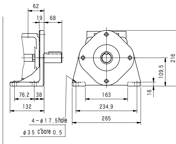
(Foot Mount)
