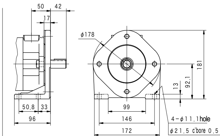
(Foot Mount)
