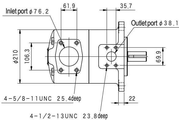
S Q P S 4 (Flange Mount)
