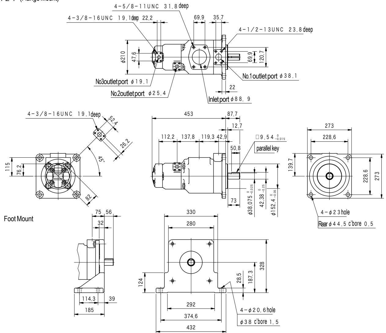
S Q P 4 2 1 (Flange Mount)
