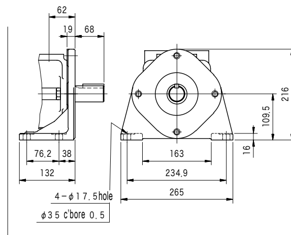
(Foot Mount)
