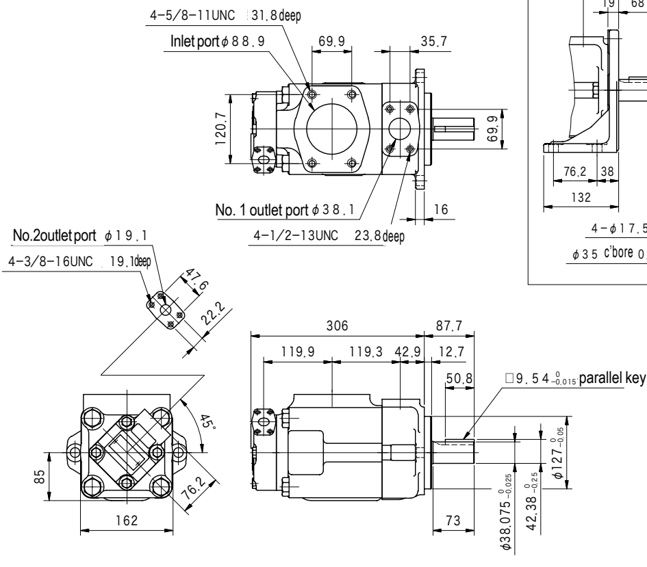
(Foot Mount)
