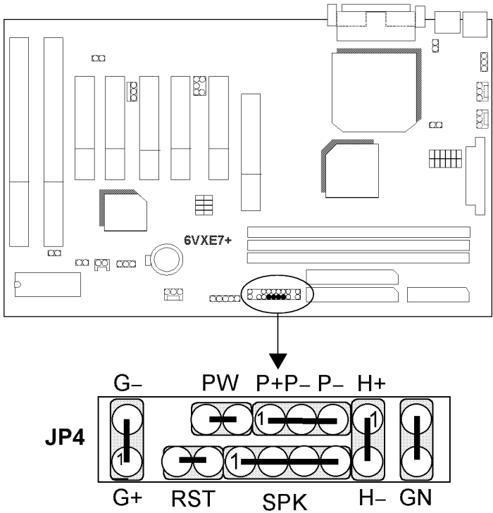
硬盘显示灯接头 (Hard Disk LED Connector) (H+H-)
