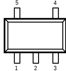
AME8840 SOT-25 Top View
