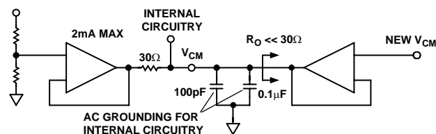
Figure 68. VCM Interface
