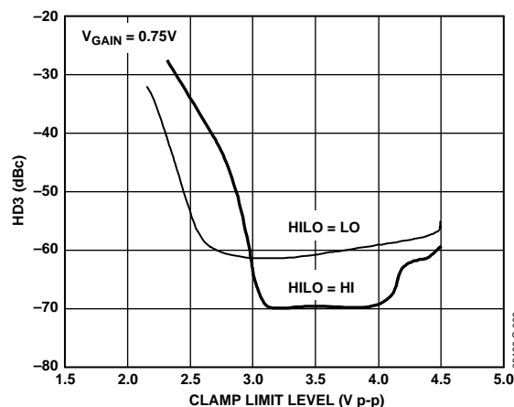
Figure 69. HD3 vs. Clamping Level for 2\text{ V p-p} Differential Input
