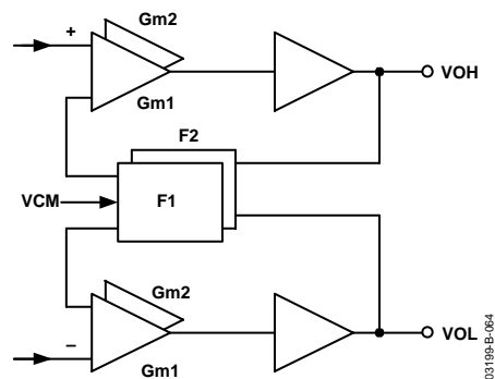
Figure 64. Postamplifier Block Diagram
