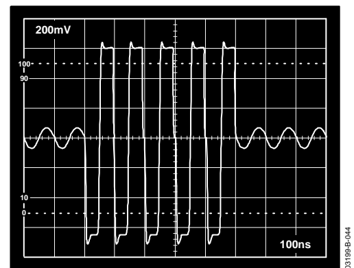
Figure 44. LNA Overdrive Recovery, V_{INH} 0.05 V p-p to 1 V p-p Burst, V_{GAIN} = 0.27 V, VGA Output Shown
