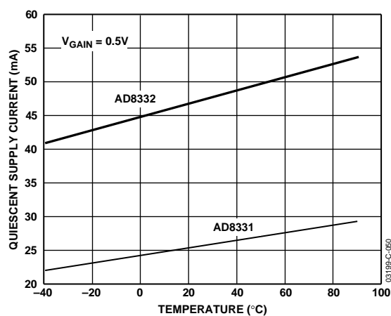
Figure 50. Quiescent Supply Current vs. Temperature
