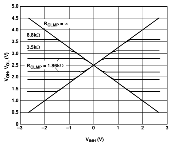
Figure 65. Output Clamping Characteristics
