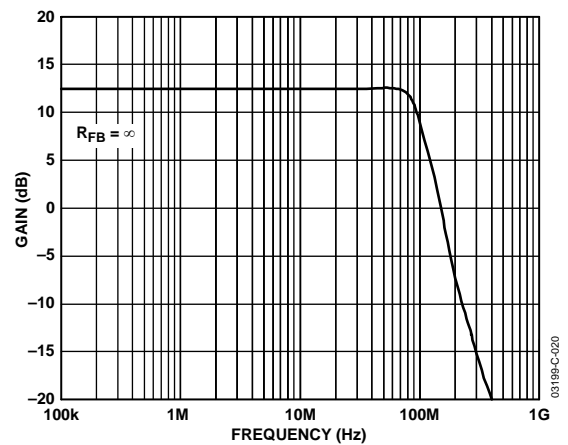
Figure 20. LNA Frequency Response, Unterminated, Single-Ended
