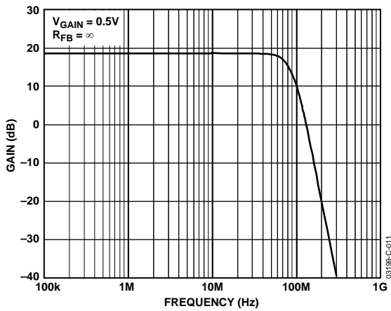
Figure 11. Frequency Response, Unterminated, R_S = 50\Omega
