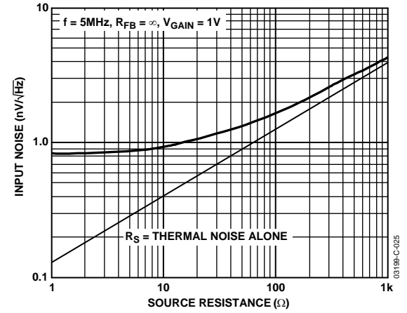
Figure 25. Input-Referred Noise vs. R_S
