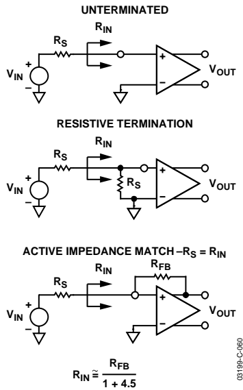
Figure 60. Input Configurations
