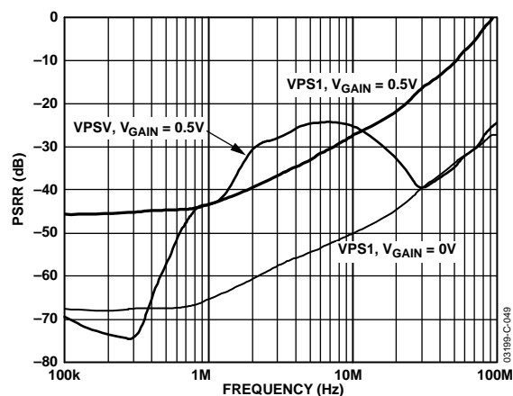
Figure 49. PSRR vs. Frequency (No Bypass Capacitor)
