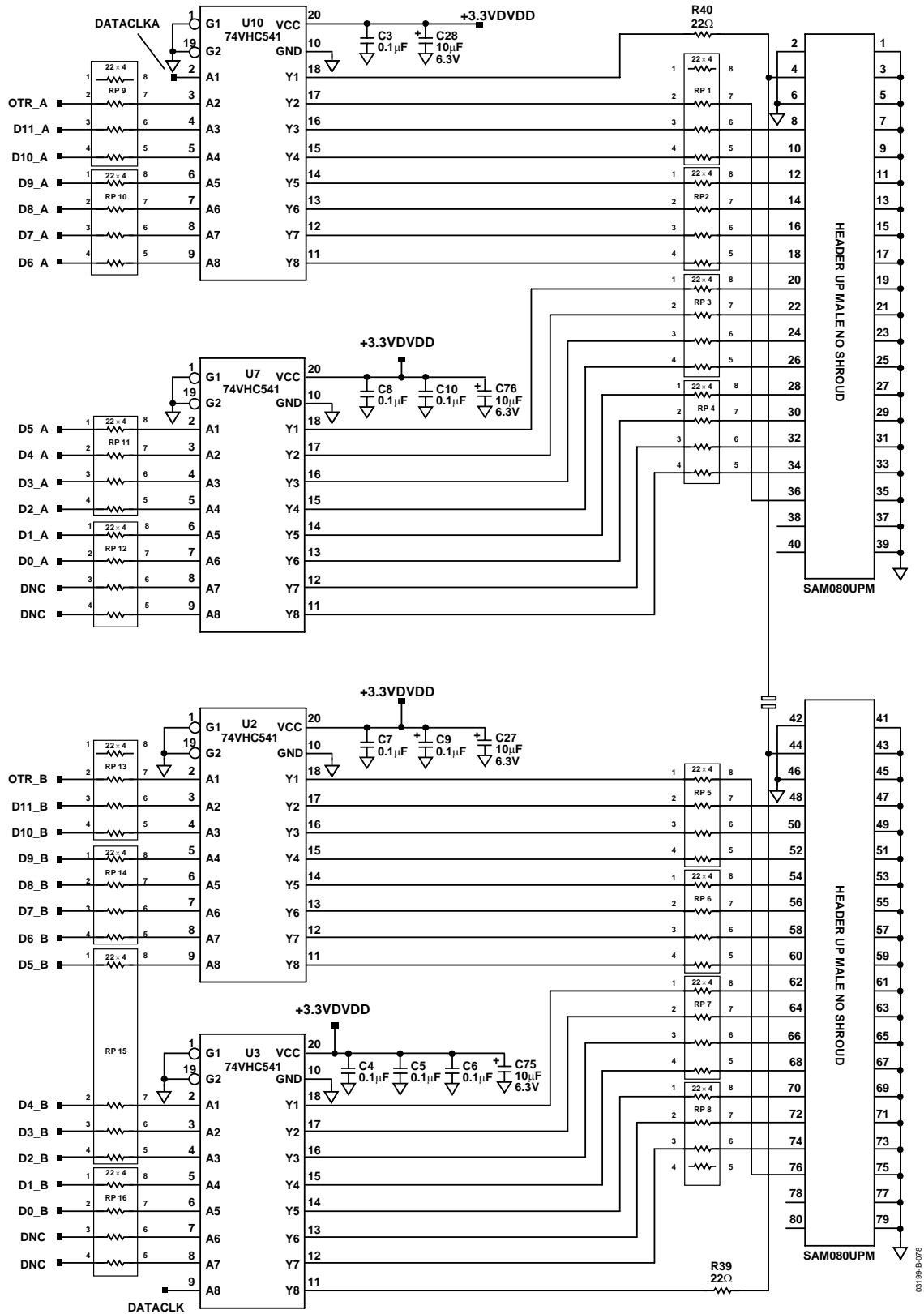
Figure 78. Interface Schematic
