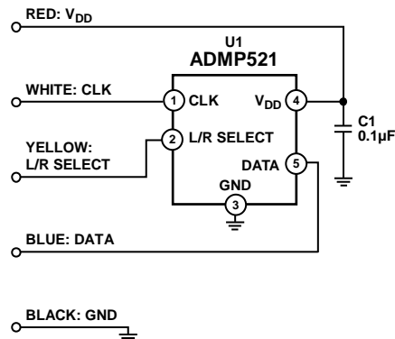
Figure 2. Evaluation Board Schematic
