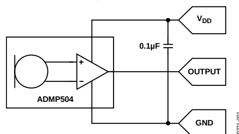
Figure 1. Evaluation Board Schematic
