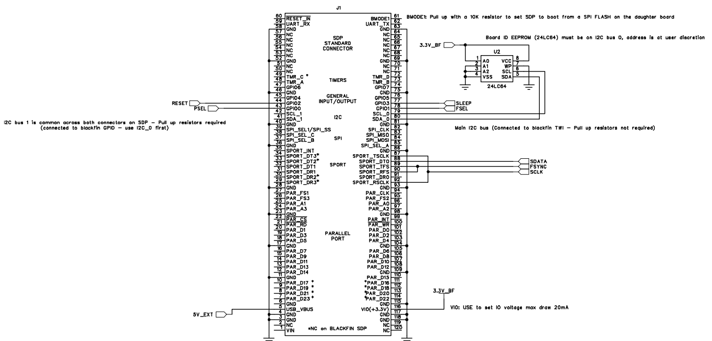
Figure 17. AD9838 Schematic Part B
