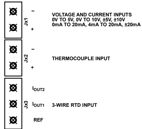
Figure 6. Input Connectors
