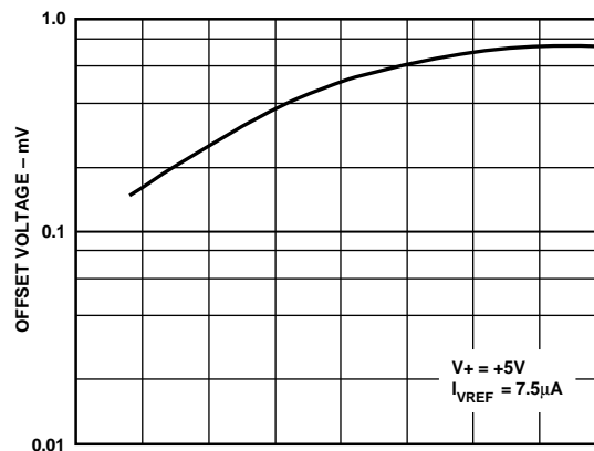
Figure 12. Set High, Set Low Input Offset Voltage vs. Temperature
