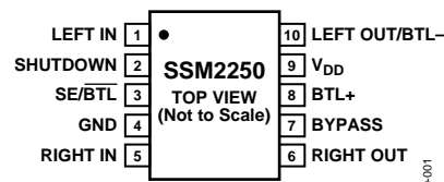
Figure 1. 10-Lead MSOP Pin Configuration (RM Suffix)
