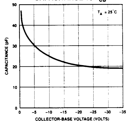
COLLECTOR-BASE CAPACITANCE vs V_{CB}
