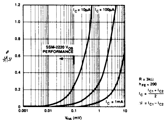
FIGURE 5b: Current Matching Accuracy % vs. Offset Voltage
