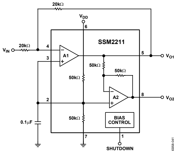
Figure 41. Simplified Schematic
