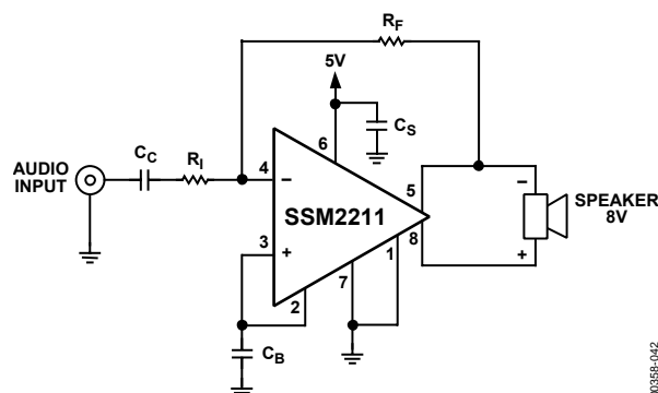
Figure 42. Typical Configuration
