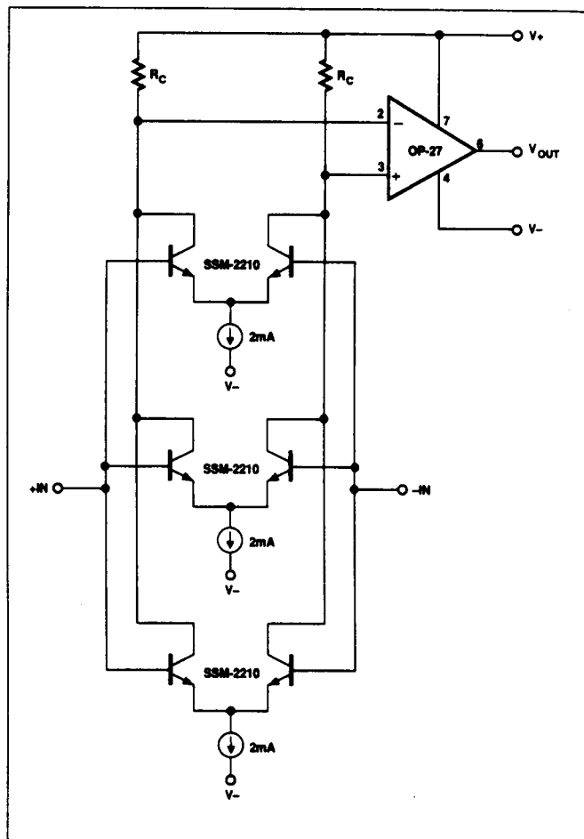
FIGURE 6: Simplified Schematic
