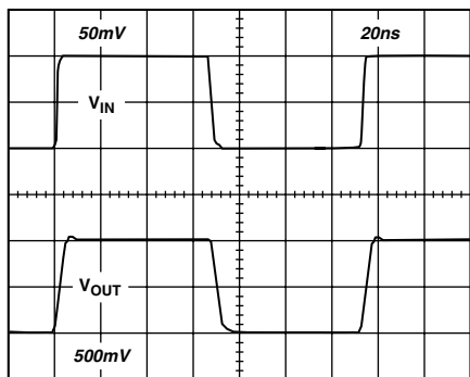
Figure 27. Small Signal Pulse Response, Gain = 10 ( R_{FB} = 400 \Omega , R_L = 150 \Omega , V_S = \pm 7.5 \text{ V} )
