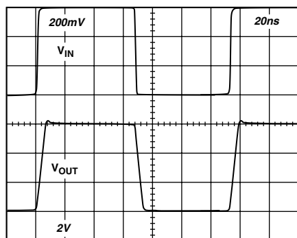
Figure 28. Large Signal Pulse Response, Gain = 10 ( R_{FB} = 400 \Omega , R_L = 150 \Omega , V_S = \pm 7.5 \text{ V} )
