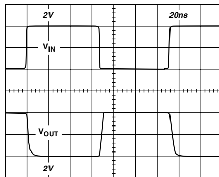
Figure 30. Large Signal Pulse Response, Gain = -1 ( R_{FB} = 909 \Omega , R_L = 150 \Omega , V_S = \pm 7.5 \text{ V} )
