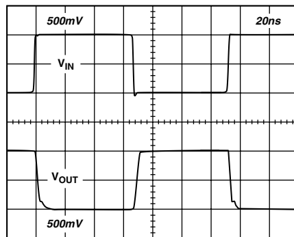
Figure 29. Small Signal Pulse Response, Gain = -1 ( R_{FB} = 909 \Omega , R_L = 150 \Omega , V_S = \pm 7.5 \text{ V} )
