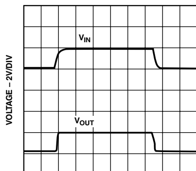
TPC 14. Turn On/Turn Off Response at 5 V, R_{LOAD} = 1.8 \text{ k}\Omega , C_{BYPASS} = 0.1 \text{ }\mu\text{F}
