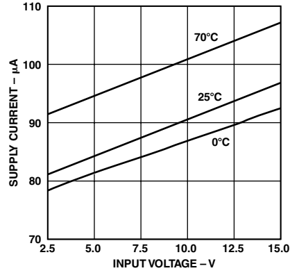
TPC 2. Supply Current vs. Input Voltage
