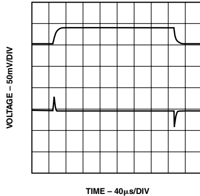
TPC 8. Line Transient Response, C_{BYPASS} = 0 \mu F
