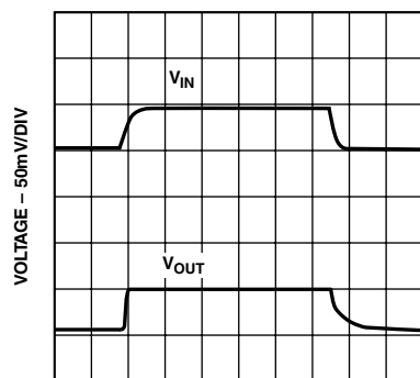
TPC 13. Turn On/Turn Off Response at 5 V, R_{LOAD} = 1.8 \text{ k}\Omega
