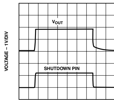
TPC 15. Shutdown Pin Response
