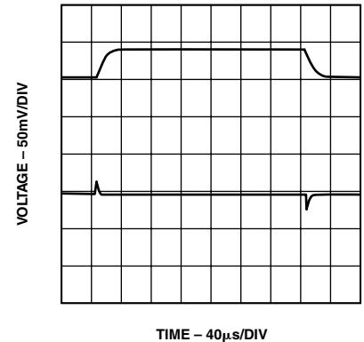
TPC 9. Line Transient Response, C_{BYPASS} = 0.1 \mu F
