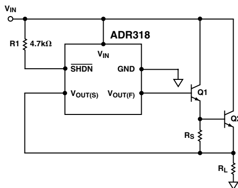
Figure 6. High Output Current with Darlington Drive Configuration
