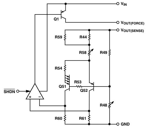
Figure 1. Simplified Schematic
