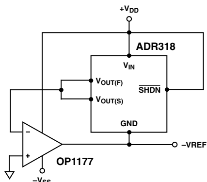
Figure 3. Negative Reference
