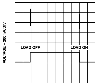
TPC 10. Load Transient Response, C_L = 0 \text{ nF}
