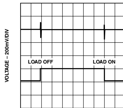
TPC 12. Load Transient Response, C_L = 100 \text{ nF}
