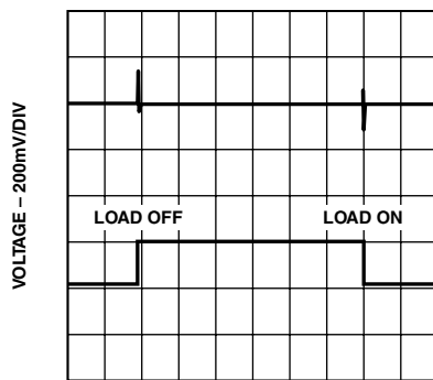
TPC 11. Load Transient Response, C_L = 1 \text{ nF}
