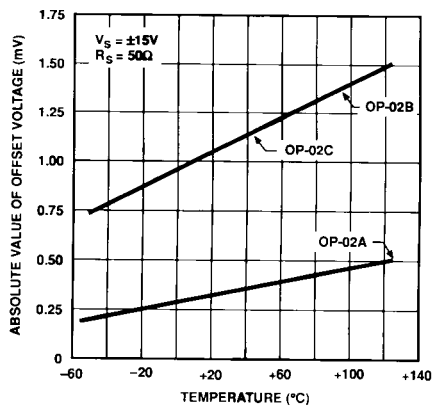
UNTRIMMED OFFSET VOLTAGE vs TEMPERATURE
