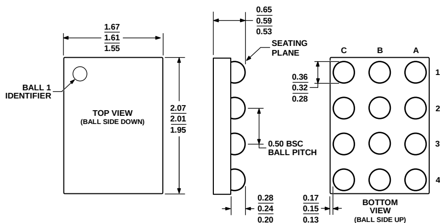
Figure 43. 12-Ball Wafer Level Chip Scale Package [WLCSP] (CB-12)
