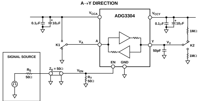
Figure 35. Capacitance at Pin Y
