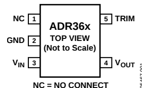
Figure 1. 5-Lead TSOT (UJ Suffix)
