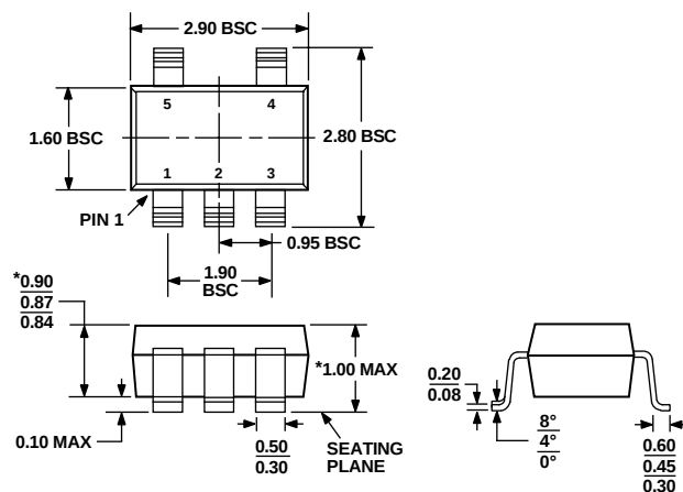
Figure 38. 5-Lead Thin Small Outline Transistor Package [TSOT] (UJ-5) Dimensions shown in millimeters
