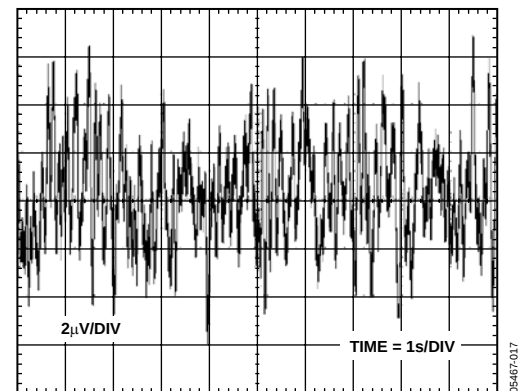
Figure 19. ADR365 0.1 Hz to 10 Hz Noise
