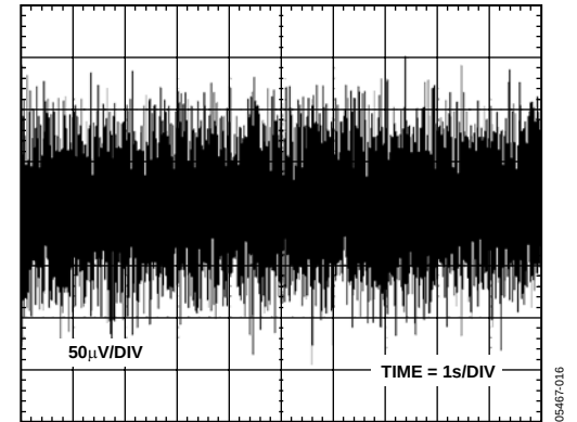
Figure 18. ADR363 10 Hz to 10 kHz Noise
