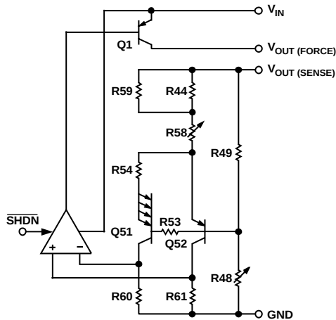
Figure 32. Simplified Schematic
