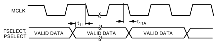
Figure 3. Control Timing
