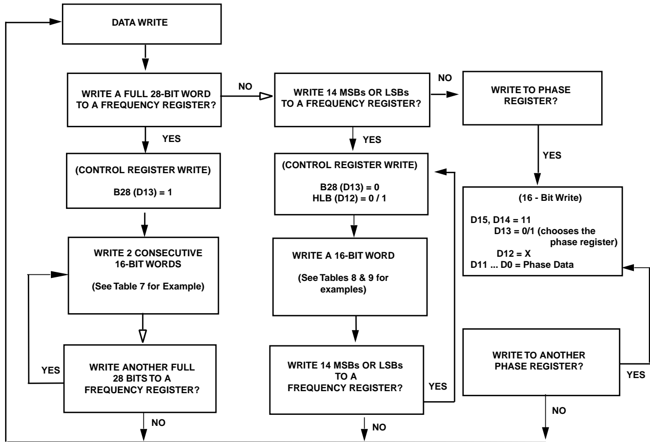
Figure 9. Data Writes
