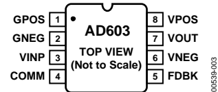
Figure 3. 8-Lead Ceramic CERDIP (Q) Package
