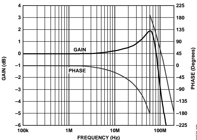
Figure 6. Frequency and Phase Response vs. Gain (Gain = -10 dB, P_{\text{IN}} = -30\text{ dBm} )
