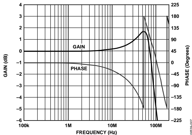
Figure 7. Frequency and Phase Response vs. Gain (Gain = +10 dB, P_{\text{IN}} = -30\text{ dBm} )
