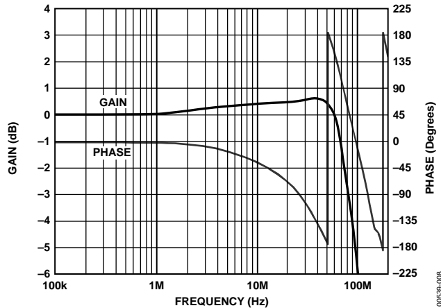
Figure 8. Frequency and Phase Response vs. Gain (Gain = +30 dB, P_{\text{IN}} = -30\text{ dBm} )
