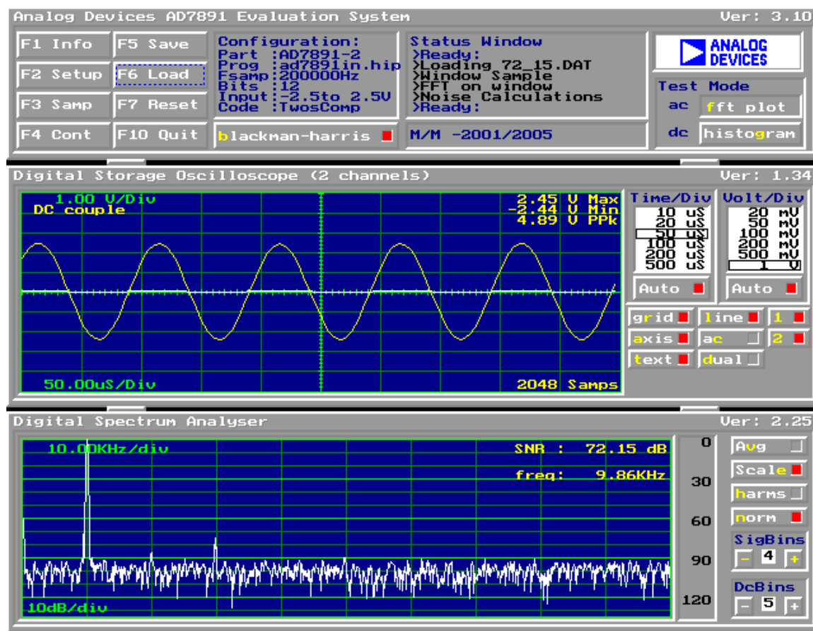
Figure 3. Main Screen
