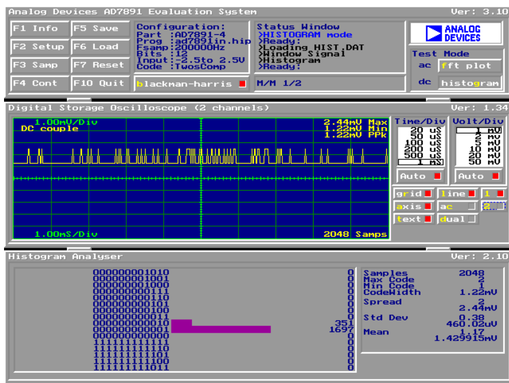
Figure 5. Histogram Screen
