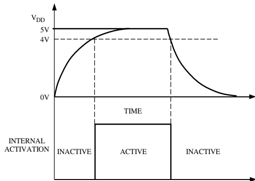
Figure 17. On-Chip Power Supply Monitor
