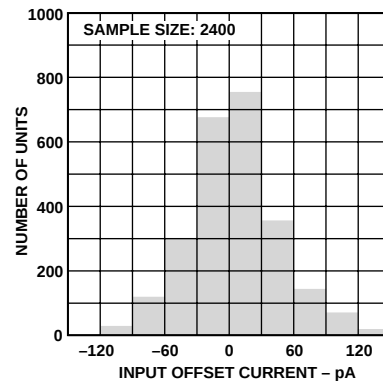
Figure 4. Typical Distribution of Input Offset Current
