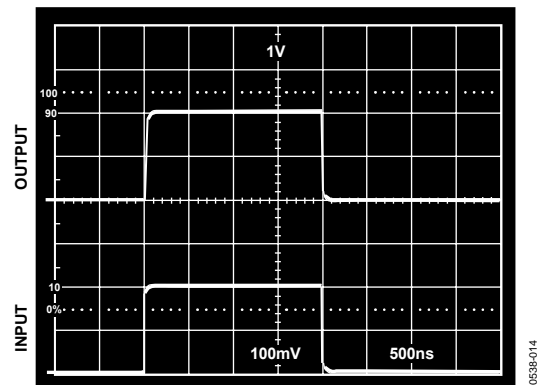
Figure 14. Transient Response, Medium and High Gain
