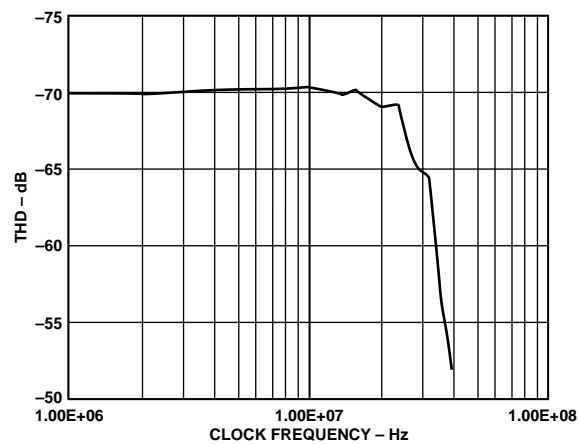
Figure 9. THD vs. Clock Frequency ( f_{IN} = 1 MHz)
