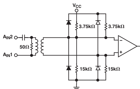
Test Circuit 4. Equivalent Analog Input
