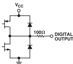
Test Circuit 2. Equivalent Digital Output
