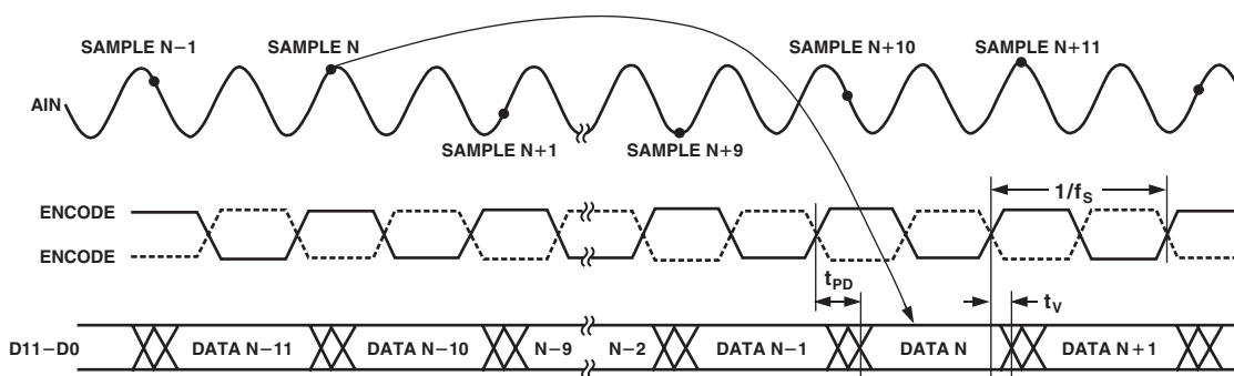
Figure 1. Timing Diagram
