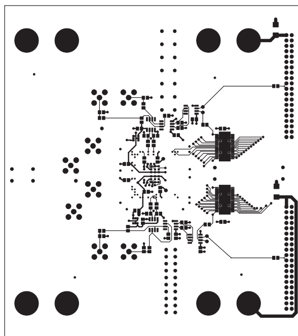
Figure 6c. Top View
